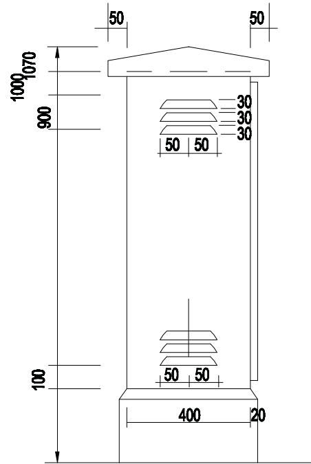
TAMPAK SAMPING
