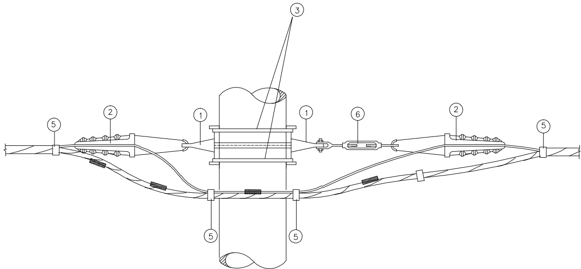
TAMPAK SAMPING
