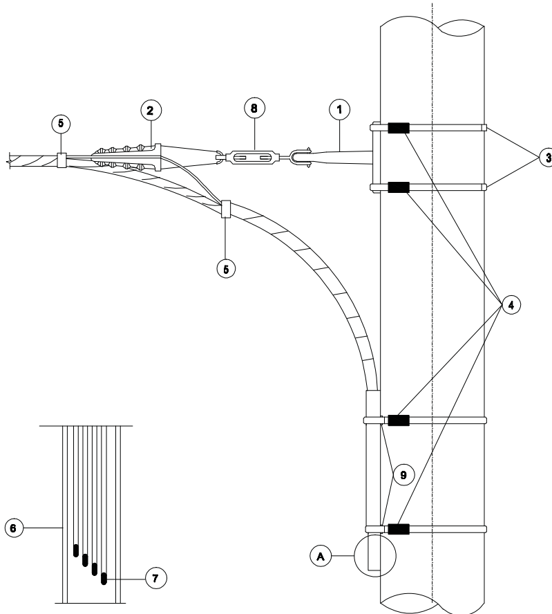
DETAIL A
