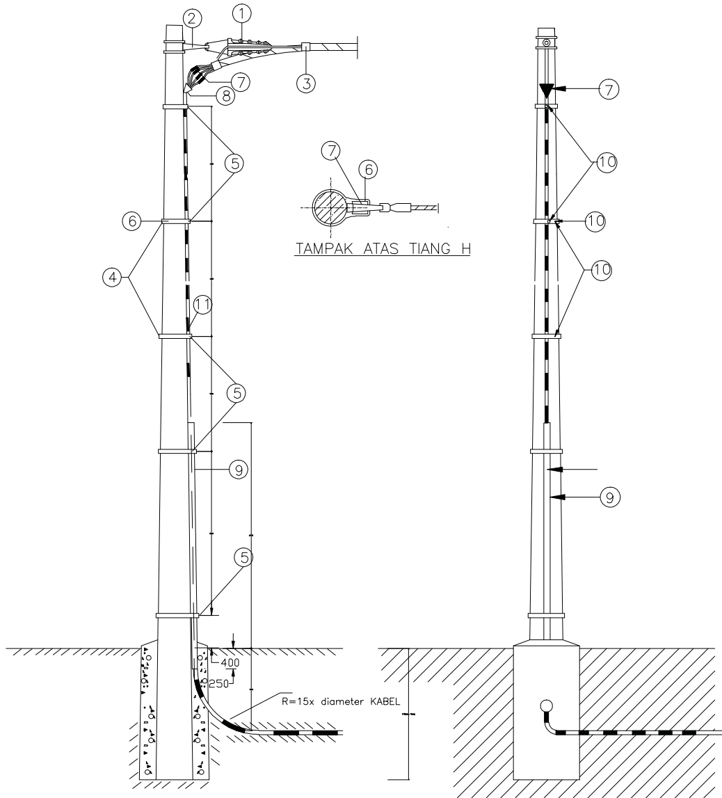
Tampak Samping
