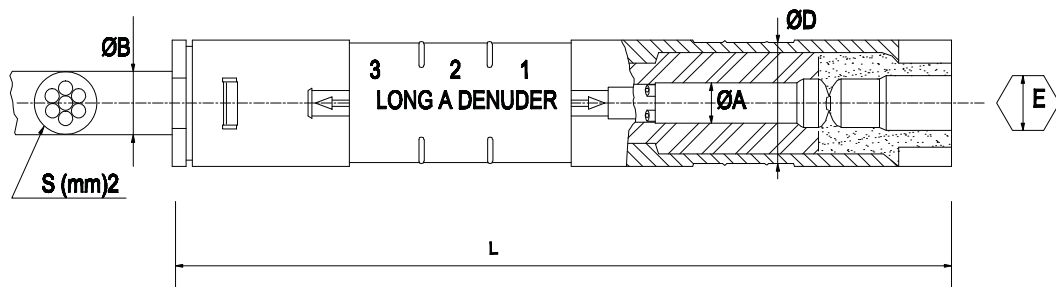
NON TENSION JOINT SLEEVE
