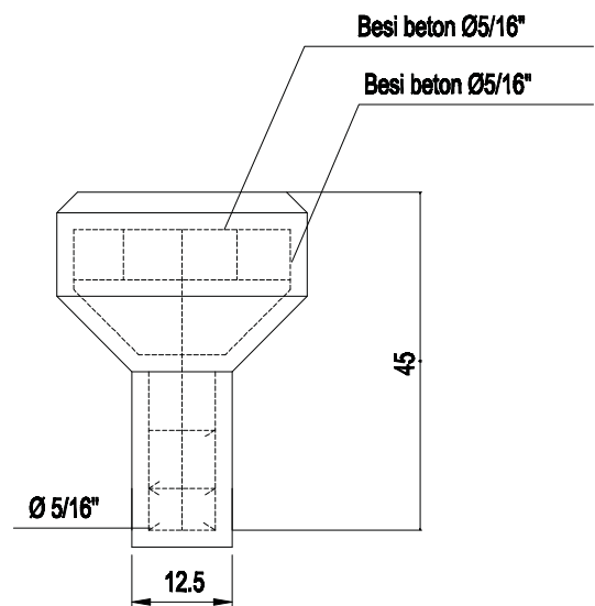
TAMPAK SAMPING
