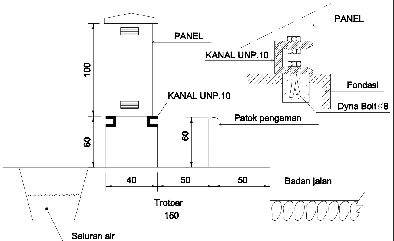
TAMPAK SAMPING
