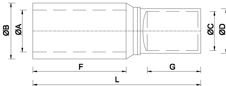
BIMETAL JUNCTION SLEEVE
