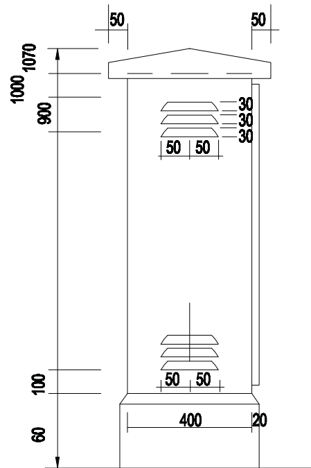
TAMPAK SAMPING
