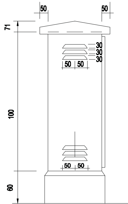
TAMPAK SAMPING
